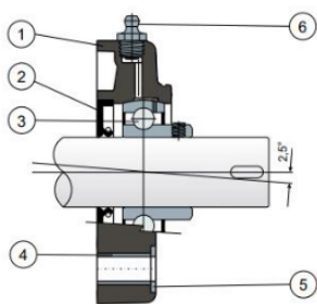
Grub screws shaft locking - Without protection cover
