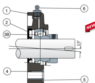
Eccentric collar shaft locking - Without protection cover
